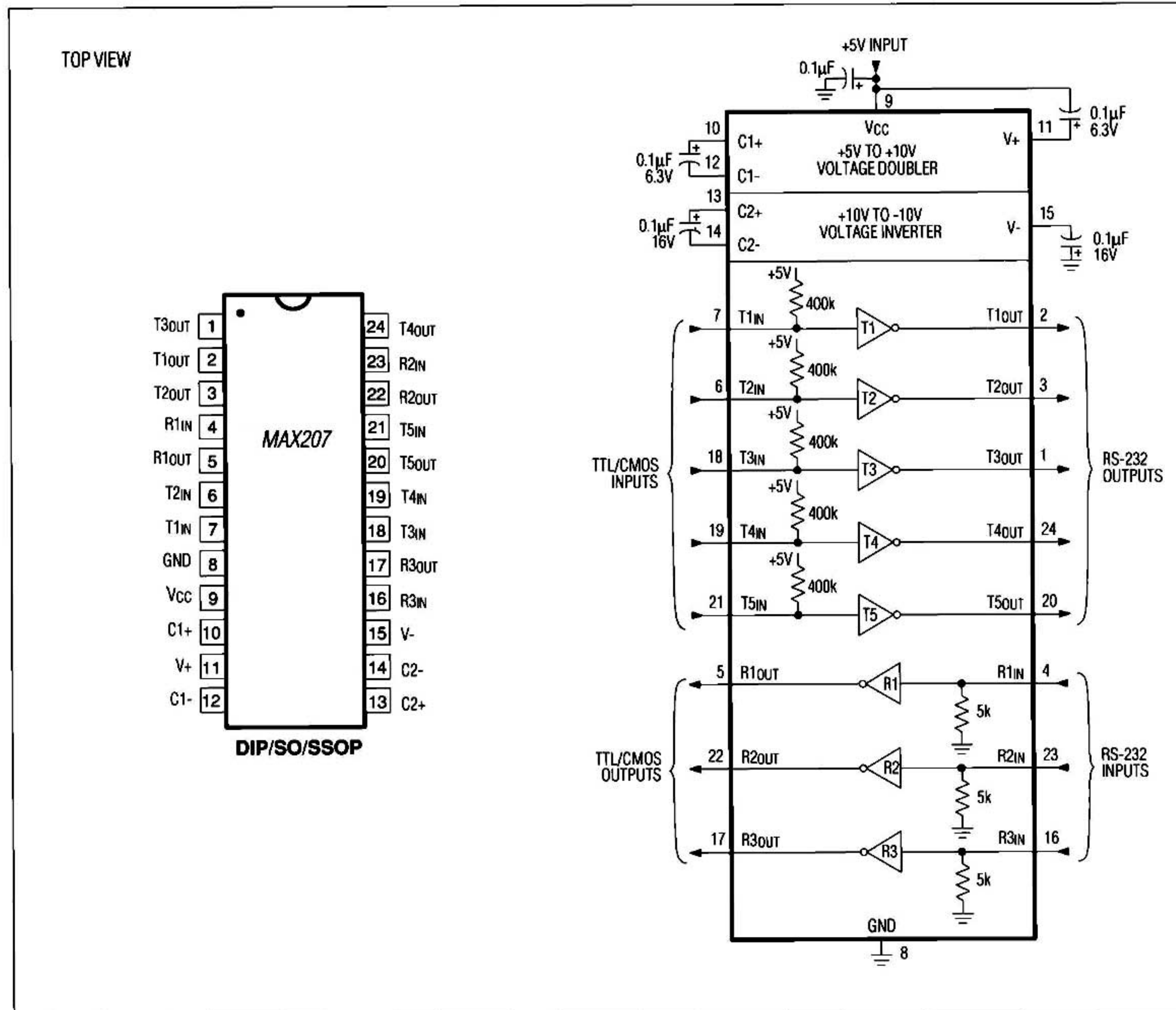
Figure 13. MAX207 Pin Configuration and Typical Operating Circuit
