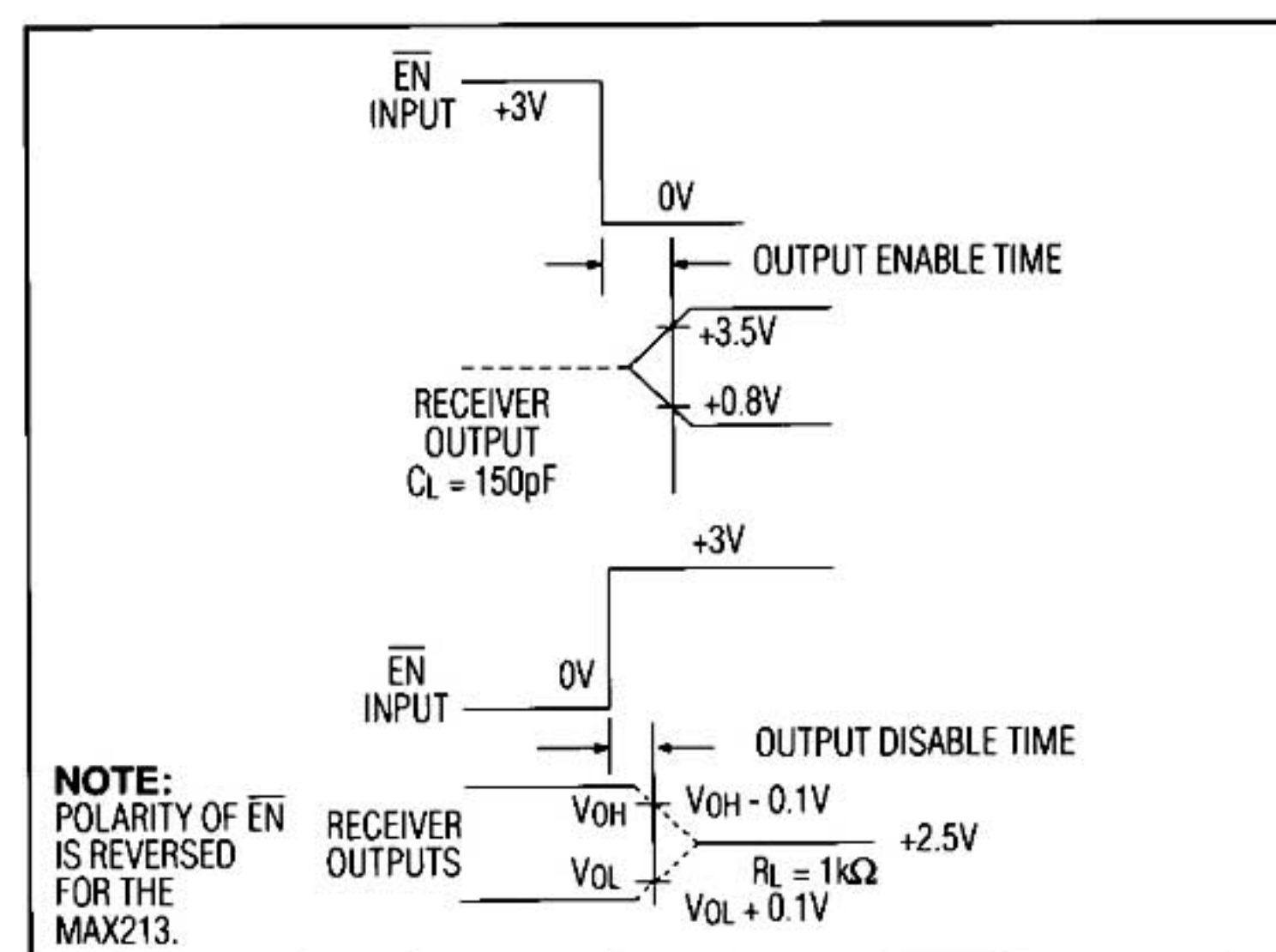
Figure 2. Receiver Output Enable and Disable Timing
