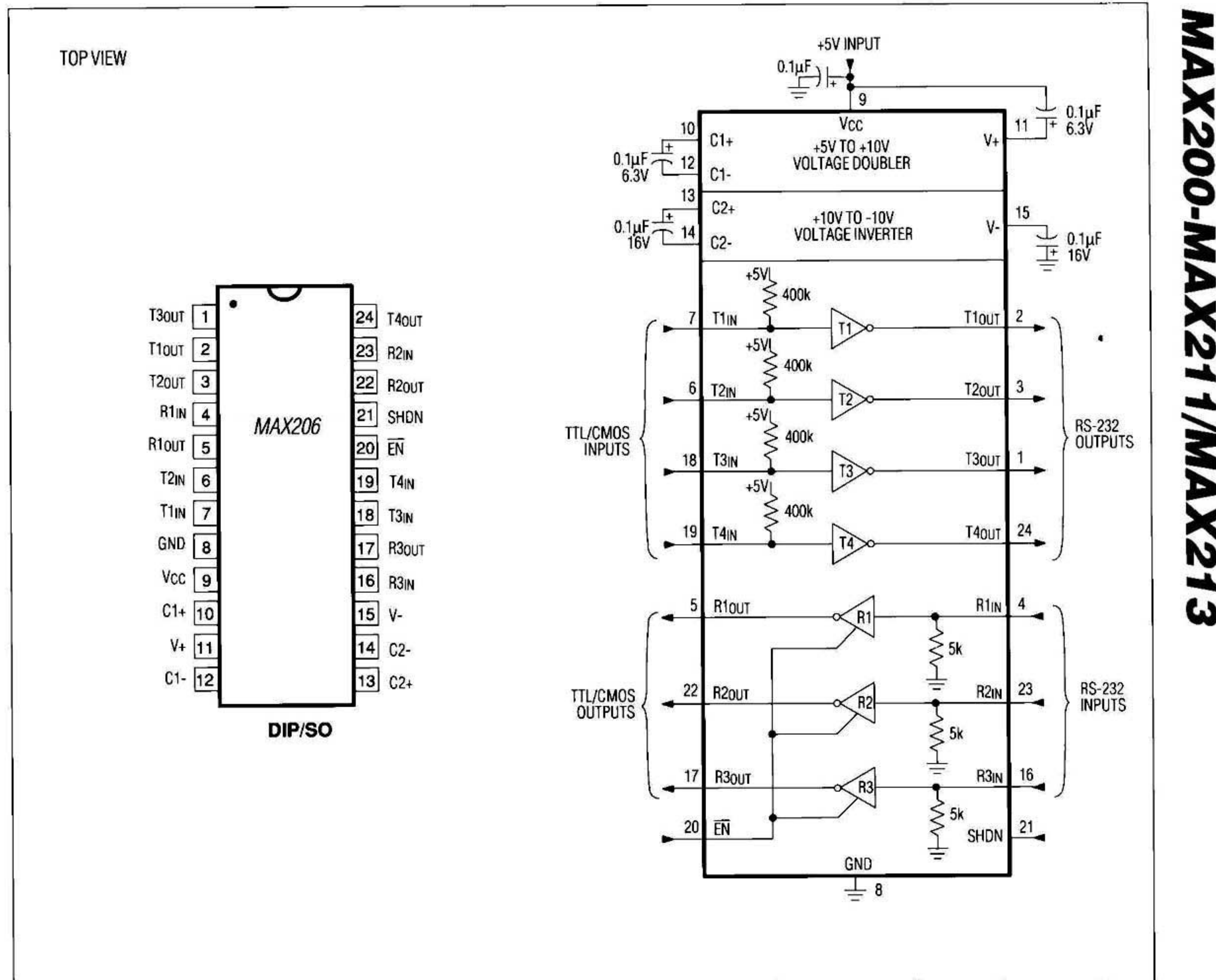
Figure 12. MAX206 Pin Configuration and Typical Operating Circuit
