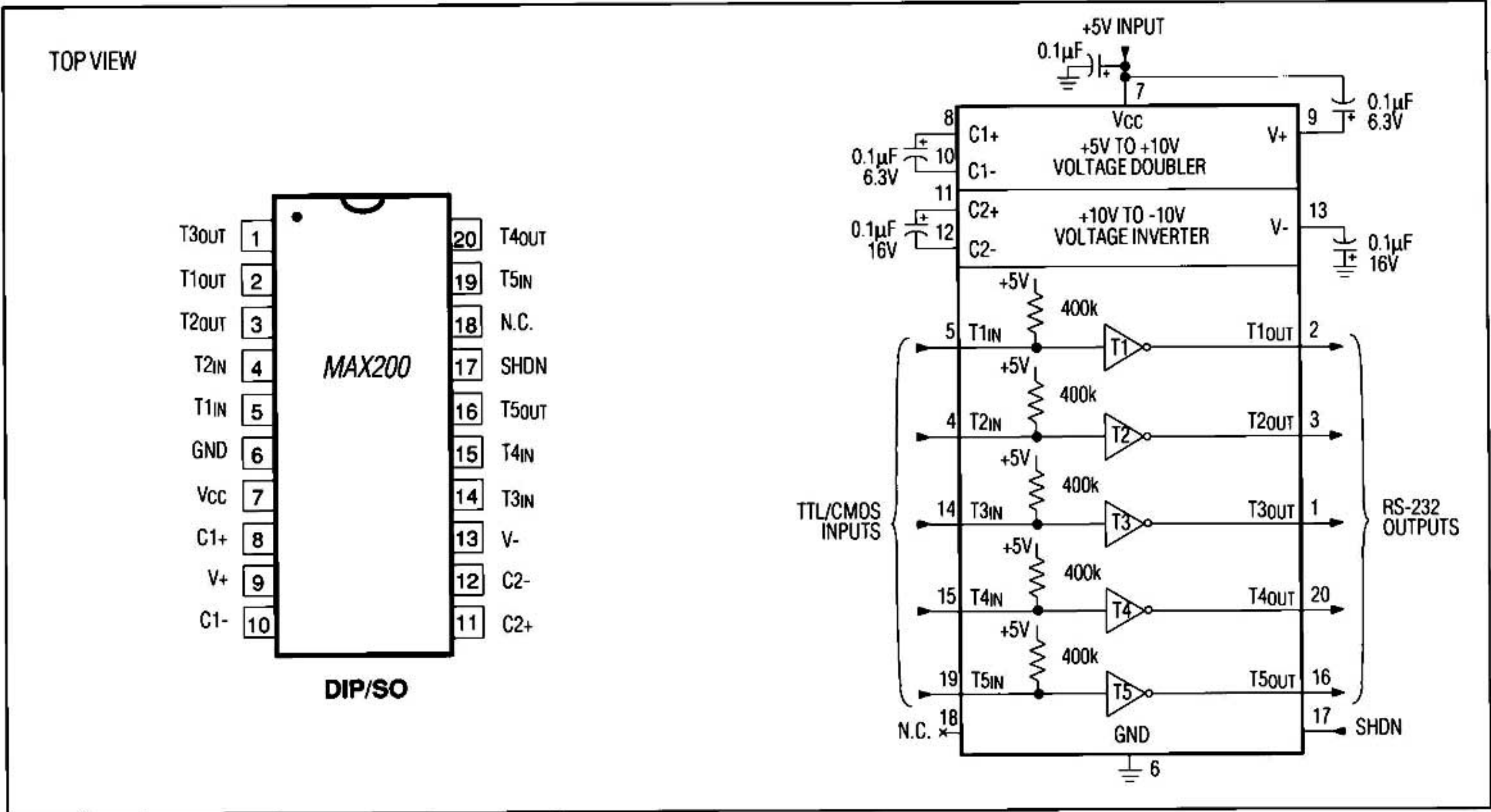
Figure 6. MAX200 Pin Configuration and Typical Operating Circuit
