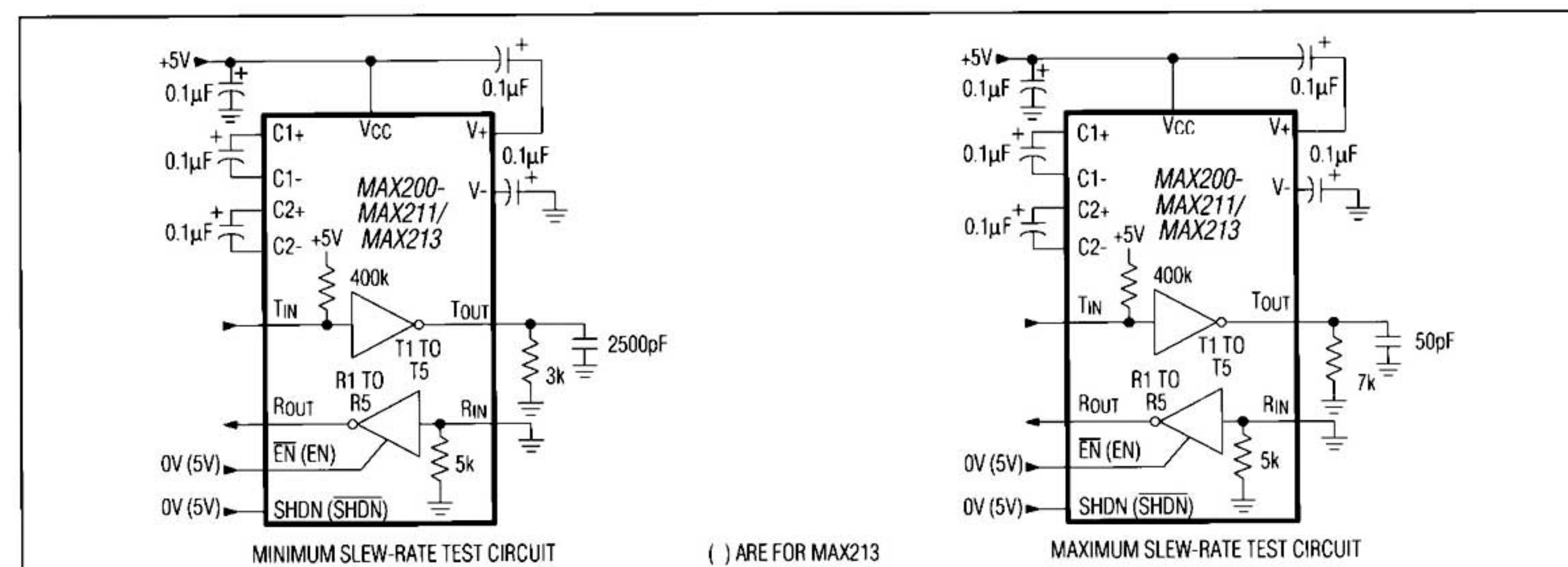
Figure 3. Transition Slew-Rate Test Circuit
