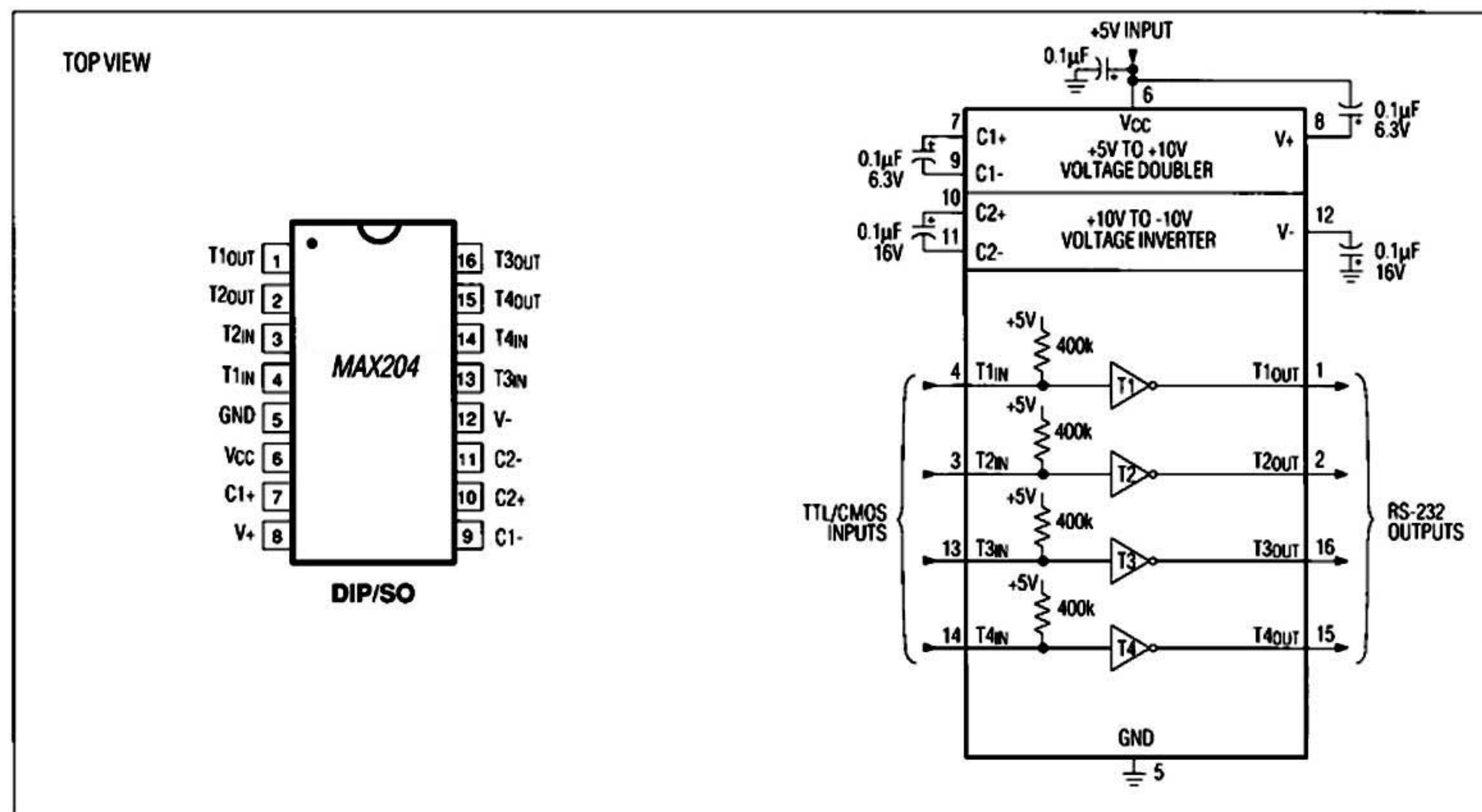
Figure 10. MAX204 Pin Configuration and Typical Operating Circuit
