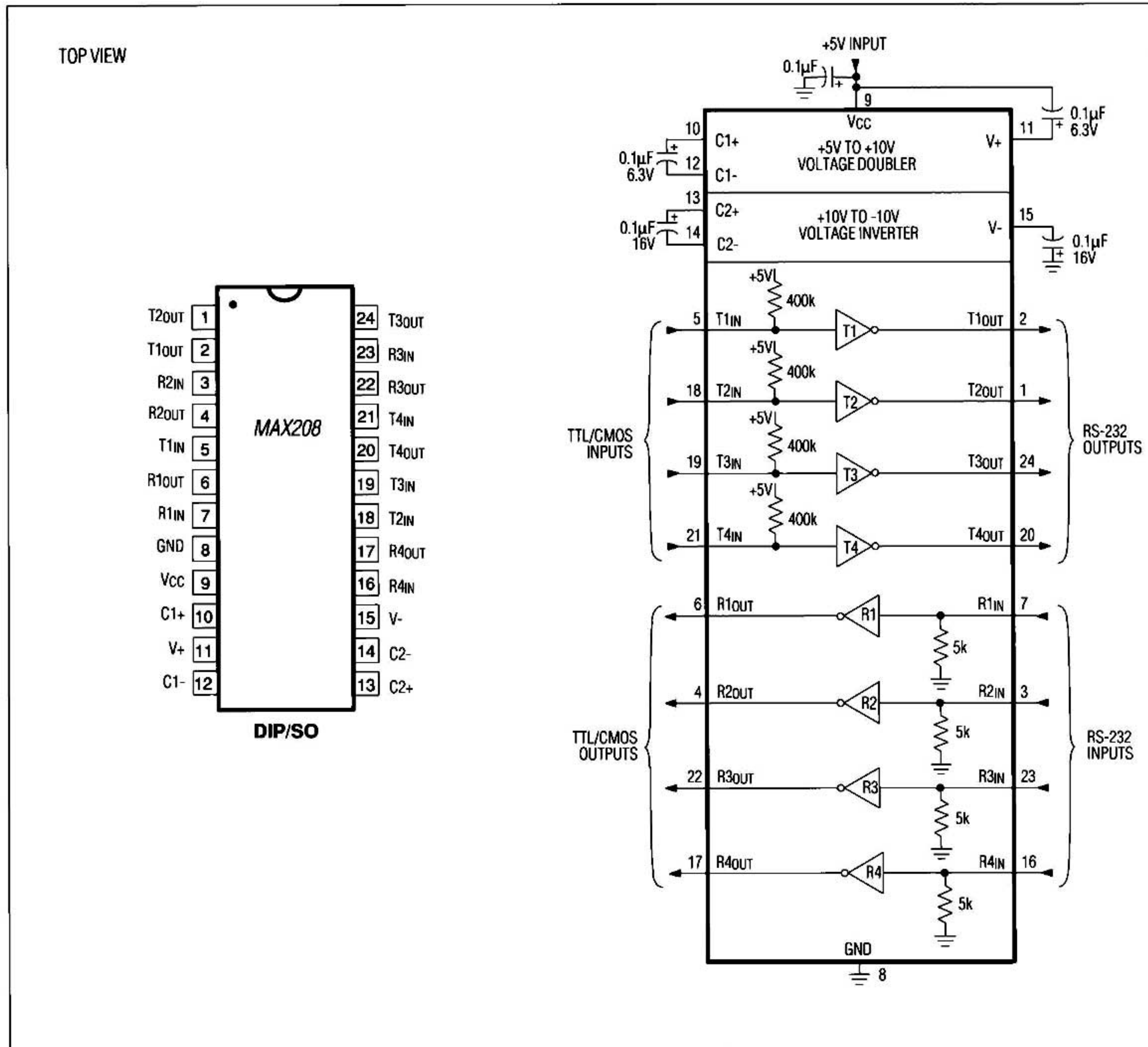
Figure 14. MAX208 Pin Configuration and Typical Operating Circuit
