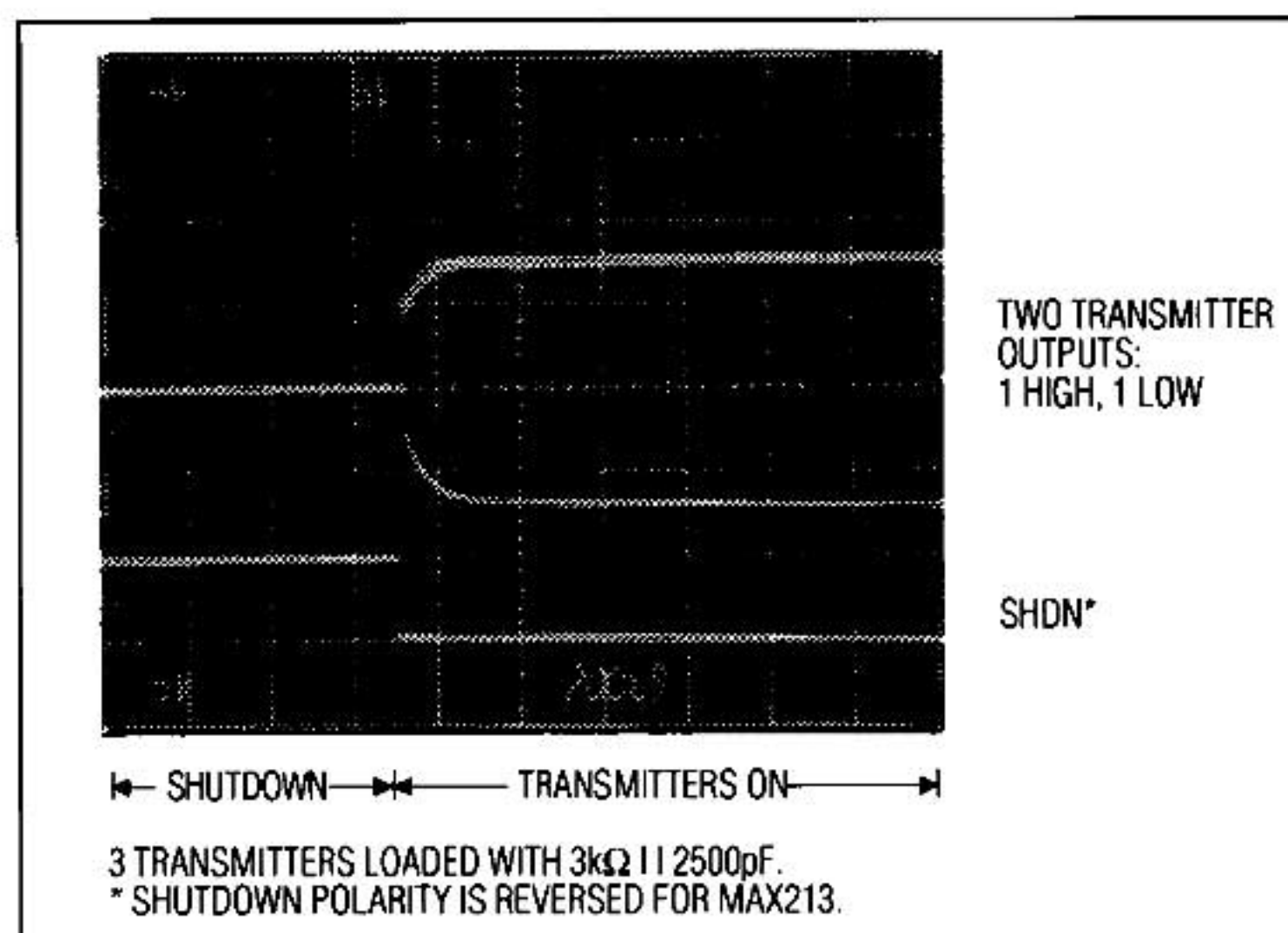
Figure 5. Transmitter Outputs When Exiting Shutdown
