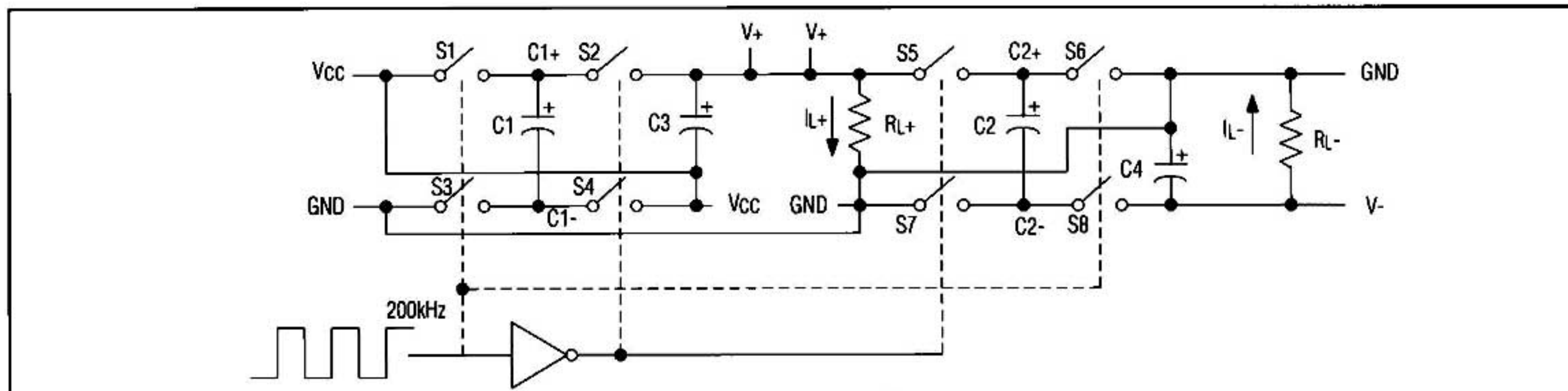
Figure 4. Dual Charge-Pump Diagram
