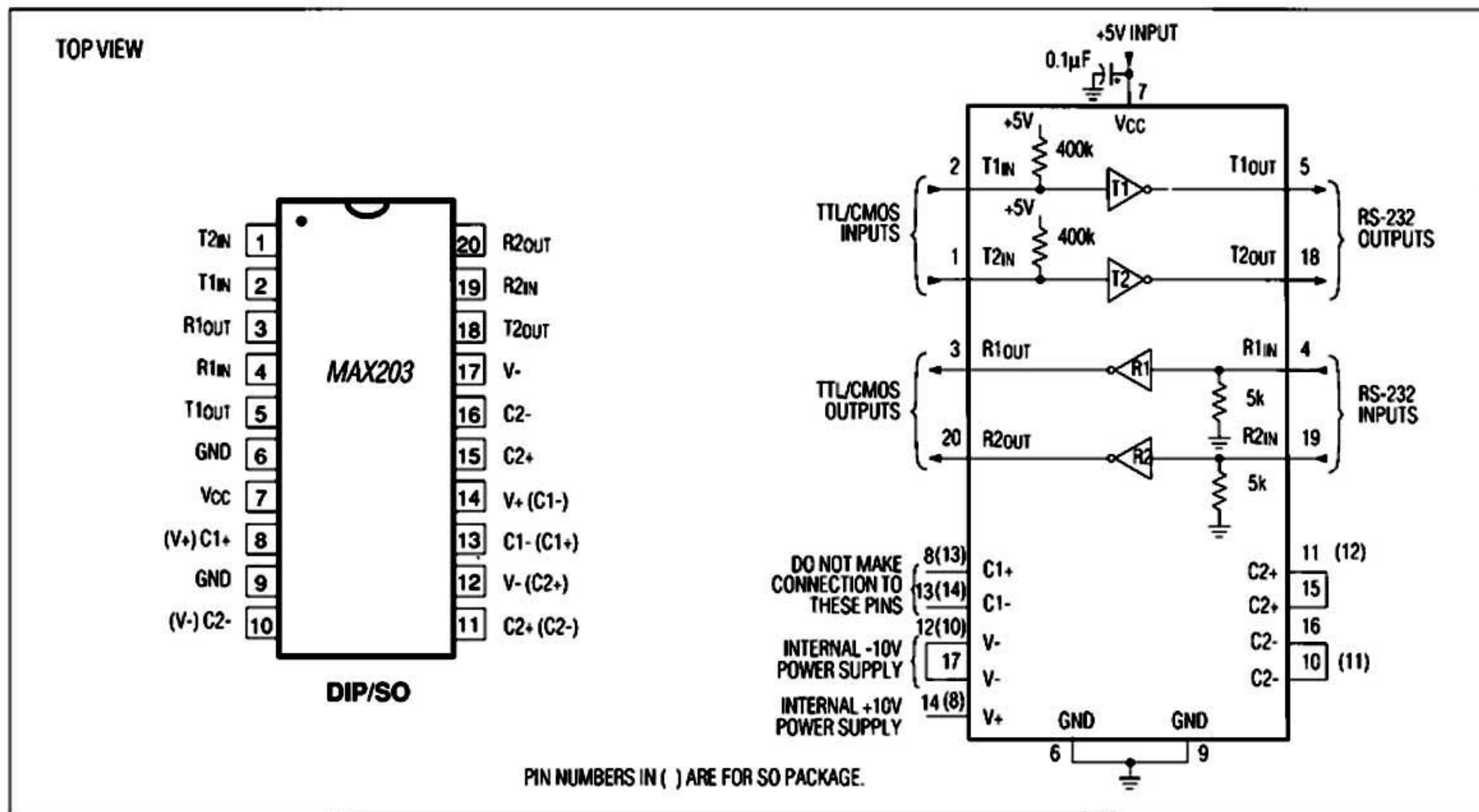
Figure 9. MAX203 Pin Configuration and Typical Operating Circuit
