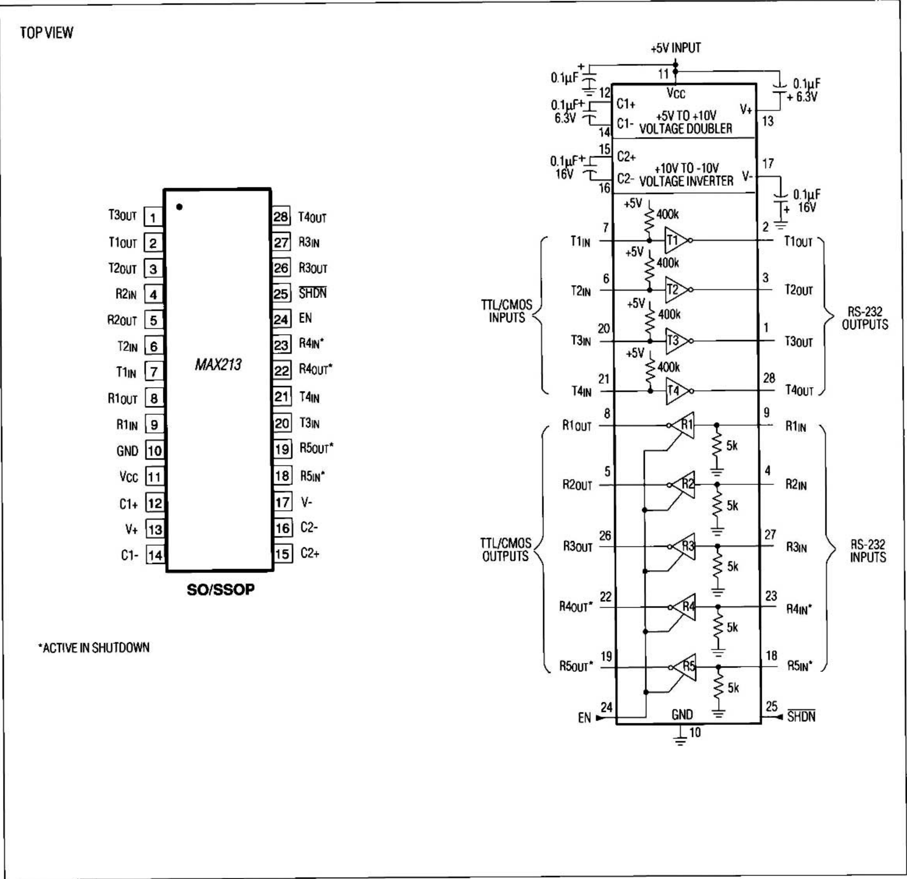
Figure 17. MAX213 Pin Configuration and Typical Operating Circuit
