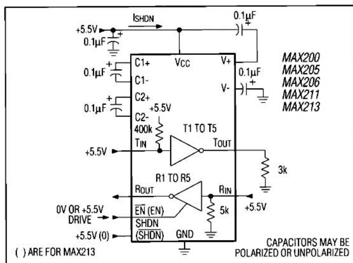
Figure 1. Shutdown Current Test Circuit
